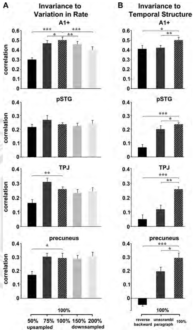
Fig. 8. Response reliability profiles from different ROIs. A: correlation of the individual responses to the intact (100%) story in an independent group of listeners ( n = 11 ) and the averaged responses to the speeded, slowed, and intact conditions ( n = 15 ) are computed. Early auditory areas exhibited high reliability in all conditions, regardless of the speed modifications. pSTG exhibited intermediate sensitivity to timing. Finally, the strongest sensitivity to stimulus rate was observed in higher order areas, such as TPJ and precuneus. B: correlation of the individual responses to the intact (100%) story and averaged unscrambled conditions (“reverse backward,” “unscrambled paragraphs,” and “unParag”) in Lerner et al. (2011). To measure the timescale of an area we scrambled a natural speech at the “words” timescale ( 0.7 \pm 0.5 s), “sentences” timescale ( 7.7 \pm 3.5 s), and “paragraphs” timescale ( 38.1 \pm 17.6 s), and then used a novel neural unscrambling procedure. In the procedure we unscrambled (reordered) the neural responses to each individual sentence (paragraph) that was presented in the scrambled sentence (paragraph) condition and we compared the unscrambled responses to the responses in the intact (100%) condition. In addition, we compared the responses to the intact story with time-reversed responses to the “backward” story (“reverse backward”). The unscrambling procedure revealed that the timescale of processing gradually increases from early sensory areas to higher order perceptual and cognitive areas. Early sensory cortices such as the primary auditory cortex (A1+) have relatively short TRWs (up to hundreds of milliseconds) and therefore respond similarly to each unit of information regardless of the scrambling level. In contrast, high order areas such as the TPJ responded differently to the same set of sentences or paragraphs when they were presented in a different order, as one would expect for an area in which the momentary response is dependent on the stimulus history over long timescales. Areas at intermediate levels of the hierarchy (e.g., pSTG) exhibited a response profile consistent with a temporal integration window of intermediate length (Lerner et al. 2011). * P < 0.05 ; ** P < 0.005 ; *** P < 0.0005 .
