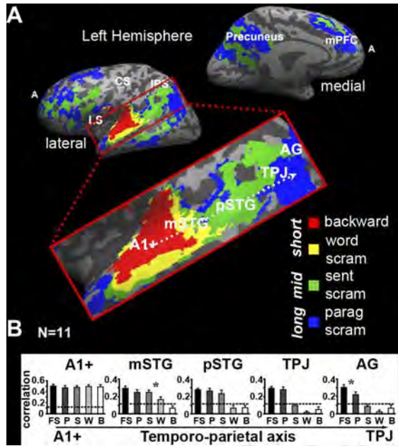
Fig. 1. Identification of regions with short and long temporal receptive windows (TRWs). A: map of TRWs, in which each voxel is colored according to the level of coherent temporal structure that was required to produce significant response reliability [intersubject correlation (inter-SC)] in that voxel. Auditory narratives of varying temporal coherence were presented: the backward stimulus has the least temporal coherence, while the word scramble, sentence scramble, and paragraph scramble stimuli contain increasing levels of temporally coherent information. Voxels are marked according to the least coherent stimulus that could drive reliable responses in that voxel. Thus voxels exhibiting reliable responses to all stimuli (including “backward”) are labeled backward and colored red (see A1+). Voxels that exhibited reliable responses to all stimuli except the backward stimulus are labeled “word scram” and colored yellow [see medial superior temporal gyrus (mSTG)]. Similarly, voxels that were reliable only for the “sentence scramble,” “paragraph scramble,” and the “intact” stimulus are labeled “sentence scram,” and they are colored green [see posterior pSTG (pSTG)]. Finally, voxels were assigned the label “paragraph scram” and colored blue if they responded reliably only to the paragraph scramble stimulus and the intact stimulus [see temporo-parietal junction (TPJ)]. B: reliability profiles for ROIs defined along the A1-TPJ axis. Early auditory areas (A1+) responded reliably to all conditions regardless of the level of temporal scrambling, and thus they have short TRWs. Areas adjacent to A1+ along the superior temporal gyrus exhibited an intermediate TRW. Here, coherent information at the “words” (mSTG), “sentences” (pSTG), or longer timescales was necessary to elicit reliable response time courses. The longest TRWs among the regions of interest (ROIs) were found in the TPJ and angular gyrus (AG). In these regions, reliable responses were evoked only by the paragraph scramble and intact stimuli.
