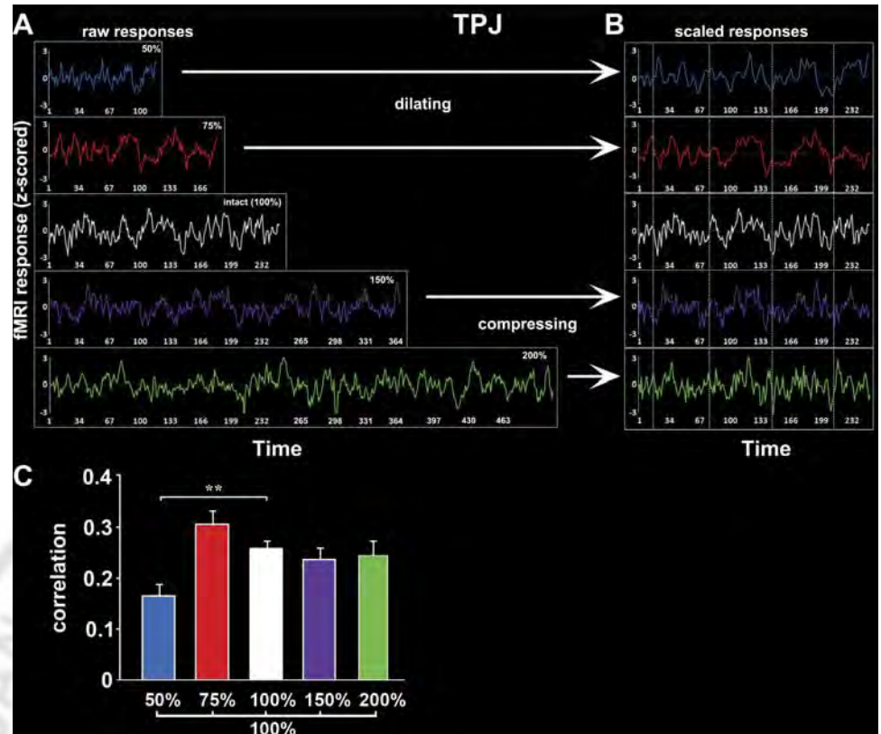
Fig. 6. Response reliability in TPJ for different presentation rates. A : raw responses in the TPJ averaged across all participants in each of the five conditions. B : dilated of the speeded 50 and 75% duration responses; and compressed of the 150 and 200% duration responses. Note that after accounting for linear response scaling, the responses to the compressed, dilated, and intact stimuli were highly correlated within TPJ. C : correlation of the individual time courses to the intact (100%) story in an independent group of listeners ( n = 11 ) and the averaged time courses to the speeded, slowed, and intact conditions ( n = 15 ).
