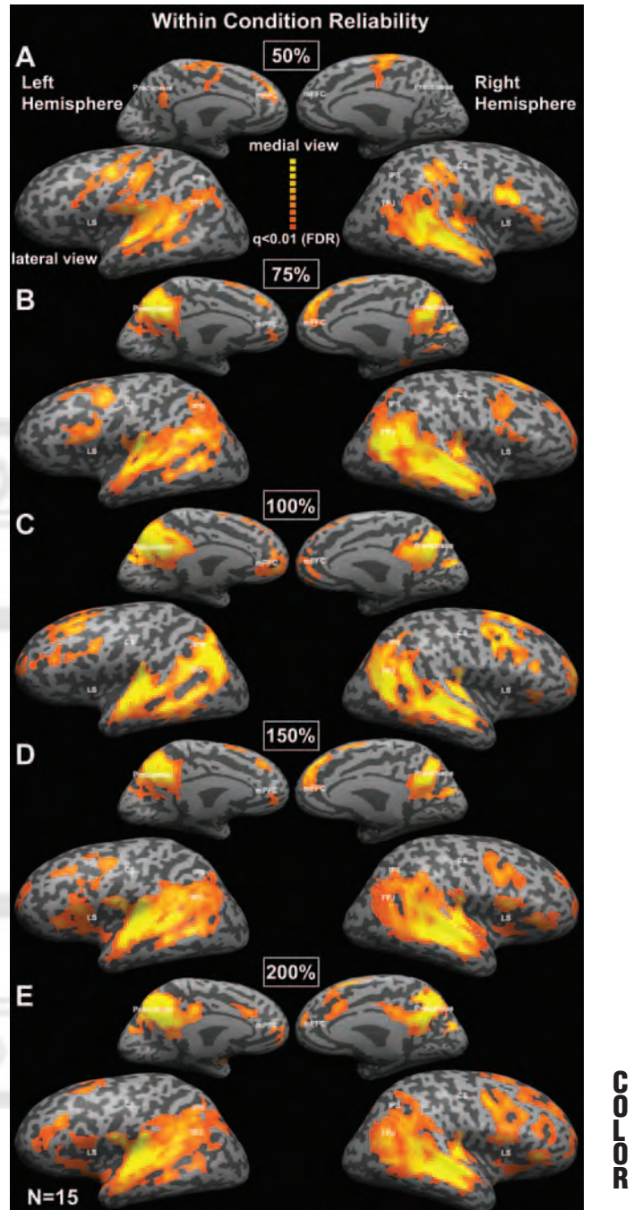
Fig. 4. Reliability of responses for each presentation rate. Maps of the reliability of responses across subjects ( n = 15 ) were computed separately for each stimulus condition and superimposed on an inflated brain shown in lateral and medial views. The maps illustrate the extent of the inter-SC for the 50% duration (A), 75% duration (B), intact story (C; 100%), 150% duration (D), and 200% duration (E). LS, lateral sulcus; CS, central sulcus; IPS, intraparietal sulcus; mPFC, medial prefrontal cortex.
