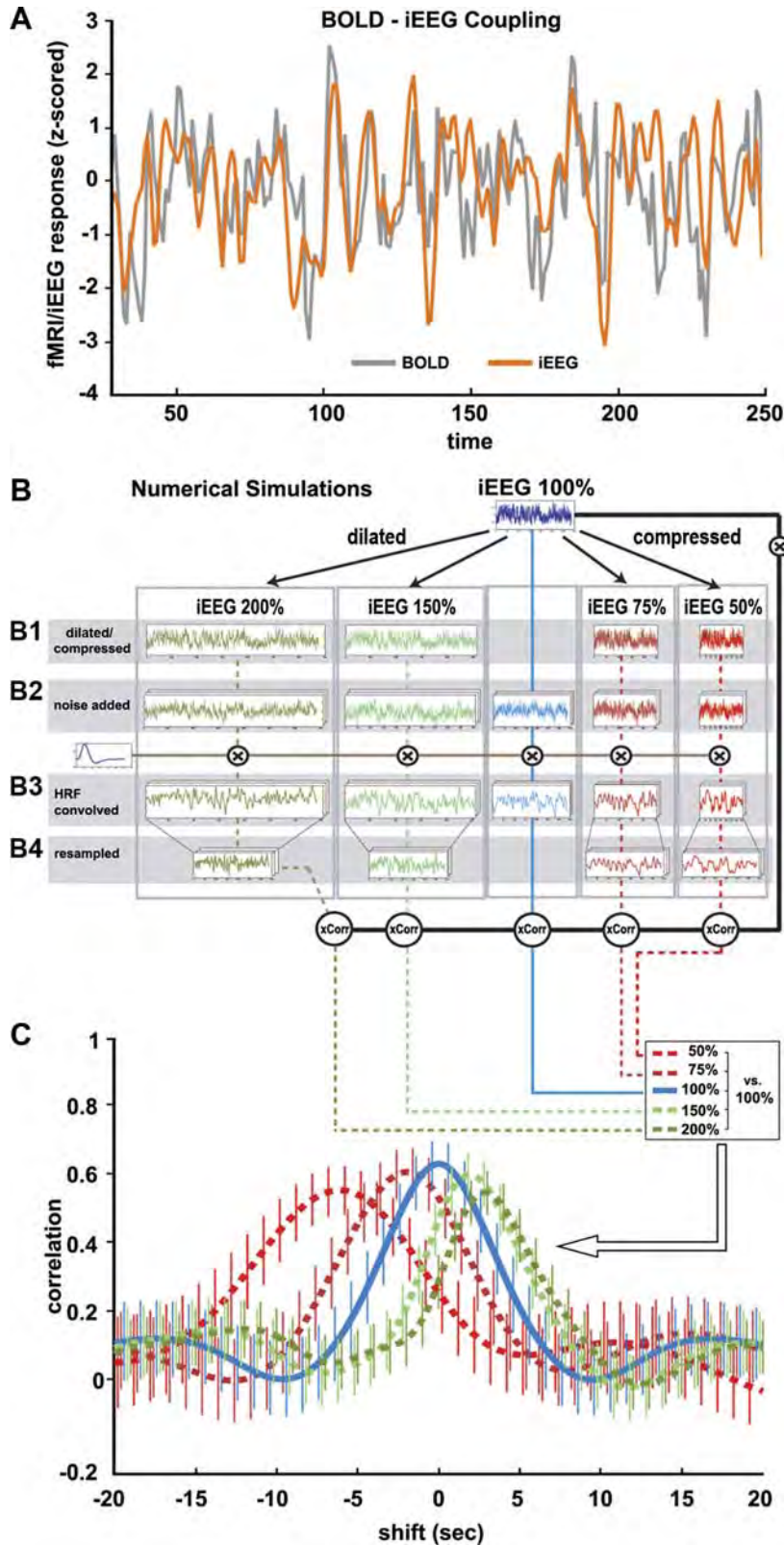
Fig. 5. Simulation pipeline and results. A : simulation is founded on strong agreement between 1) the downsampled and convolved intracranial-EEG (iEEG) power recorded from an electrode at the lateral Sylvian fissure in an individual epileptic patient listening to the 100% condition, and 2) averaged blood-oxygenation level-dependent (BOLD) responses sampled from the same area in healthy individuals hearing the 100% condition. The strong agreement between the signals is striking given that the BOLD and iEEG signals were acquired from different subjects and different experimental setups. FMRI, functional MRI. B : modeling steps: the electrophysiological response was downsampled (or upsampled) to mimic a linear scaling of the neural signal in response to differing stimuli ( B1 ). Spectrum-matched noise was added to the signals to produce simulated BOLD correlation values which match those obtained empirically ( B2 ). Noisy rescaled iEEG signals were then convolved with an a hemodynamic response function (HRF; B3 ). Next, the compressed (or dilated) BOLD response time courses were upsampled (or downsampled) to the same time-base as the BOLD responses to the 100% duration story ( B4 ). C : cross-correlation of the HRF-convolved speeded (slowed) iEEG signals and the HRF convolved original iEEG signal, after up (down) sampling. The results of the simulation procedure indicate that in cases where the underlying neural responses are linearly scaled, the upsampled and downsampled BOLD signals will be highly correlated with the convolved original signal but with a phase lag.
